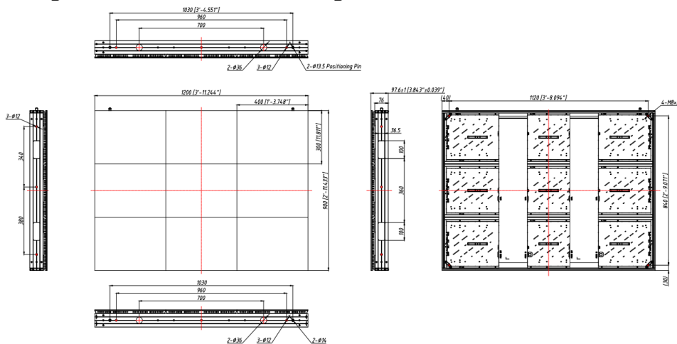
Figure 2 1200*900mm Drawing of Rear Maintenance Cabinet
