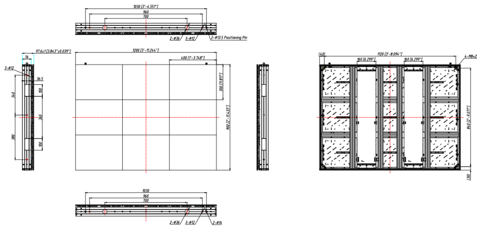
Figure 1 1200*900mm Drawing of Front Maintenance Cabinet
