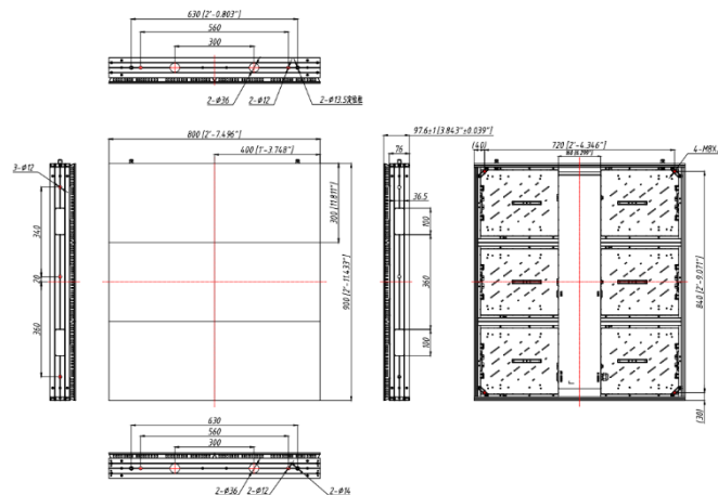
Figure 2 800*900mm Drawing of Rear Maintenance Cabinet
