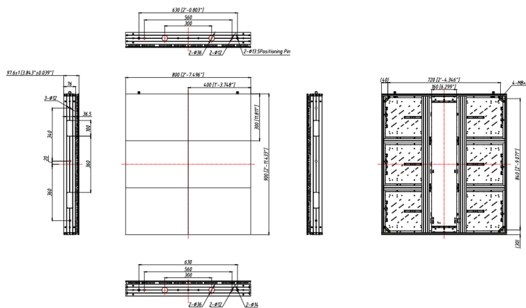
Figure 1 800*900mm Drawing of Front Maintenance Cabinet
