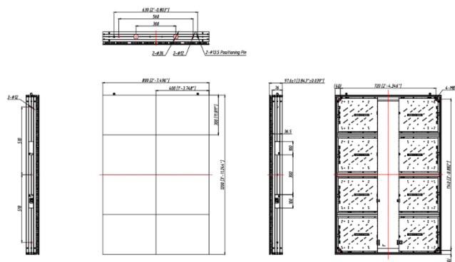
Figure 1 800*1200mm Drawing of Front Maintenance Cabinet
