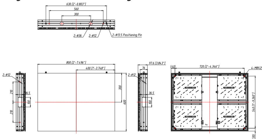
Figure 2 800*900mm Drawing of Rear Maintenance Cabinet
