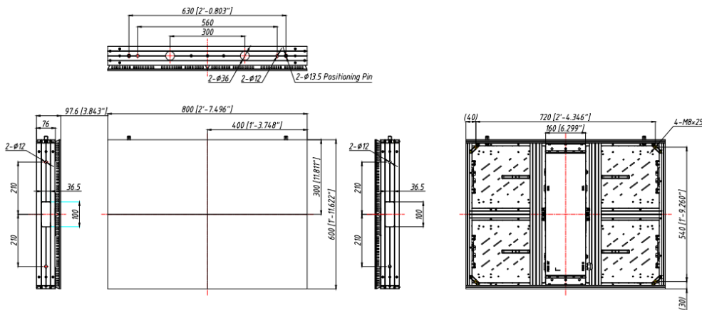
Figure 1 800*900mm Drawing of Front Maintenance Cabinet
